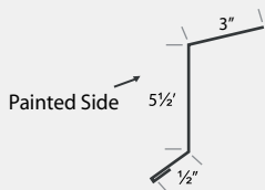
LONG EAVE TRIM
