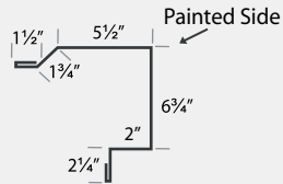
HR GABLE
