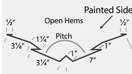
CLEAT
