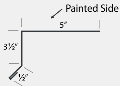
SHORT EAVE TRIM
