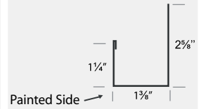
HR J-CHANNEL
