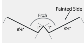
VALLEY FLASHING
