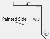
CLEAT
