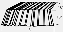
HR FORMED RIDGE CAP
