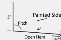
OPEN HEM ENDWALL / SIDEWALL
