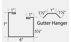
HR GUTTER
