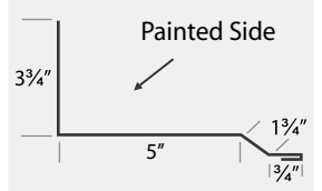
HR TRANSITION
