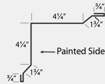
HR INSIDE CORNER
