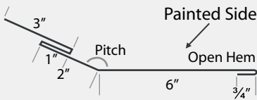
OPEN HEM TRANSITION
