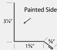
HR BASE TRIM
