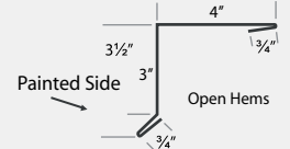
OPEN HEM GABLE
