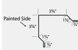
HR OUTSIDE CORNER
