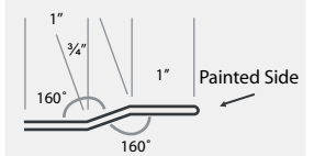
VALLEY CLEAT
