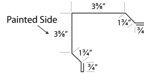
HR OUTSIDE CORNER
