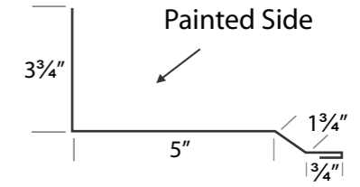
HR TRANSITION
