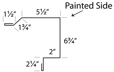
LONG EAVE TRIM
