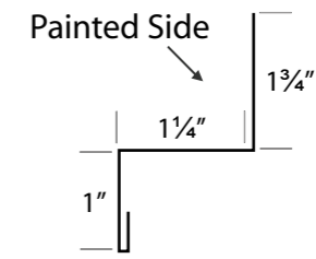
HR DOUBLE ANGLE
