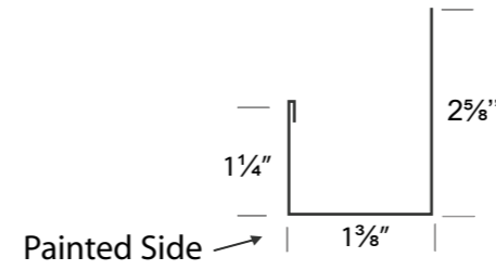
HR J-CHANNEL
