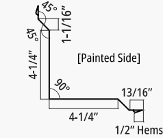
LR Inside Corner
