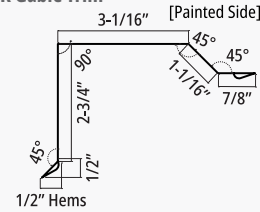
LR Gable Trim
