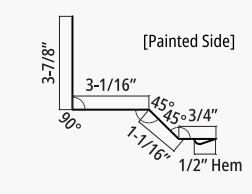
LR Step Sidewall Flashing
