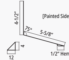
LR Endwall/Sidewall Flashing
