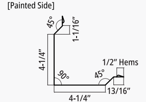
LR Outside Corner
