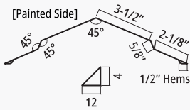
LR Hip Cap
