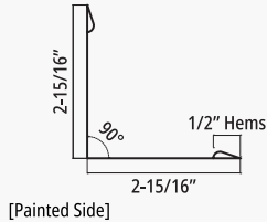
LR Angle 3"x3"
