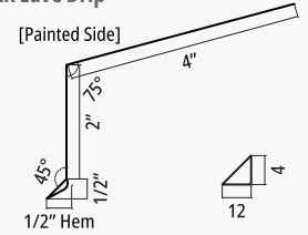
LR Eave Drip
