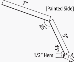
LR Gambrel Flashing
