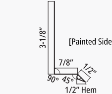
LR Base Trim
