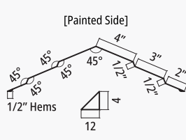
LR 20" Ridge Cap
