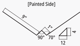
LR Transition Flashing
