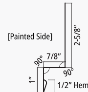
LR Double Angle Flashing
